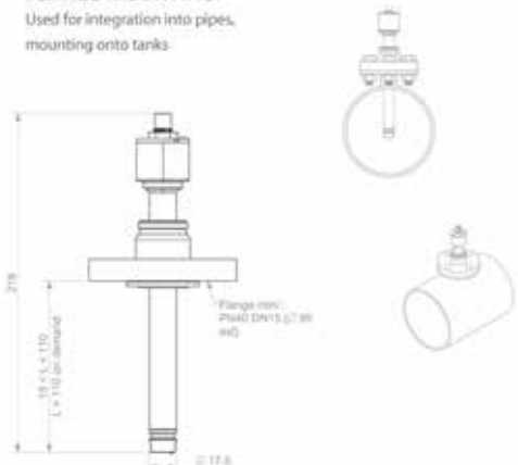
Mounting Options of Density and Viscosity Sensor
