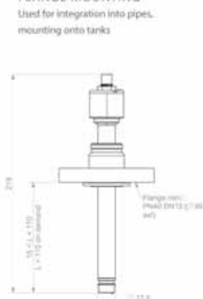
Mounting Options of Density and Viscosity Sensor
