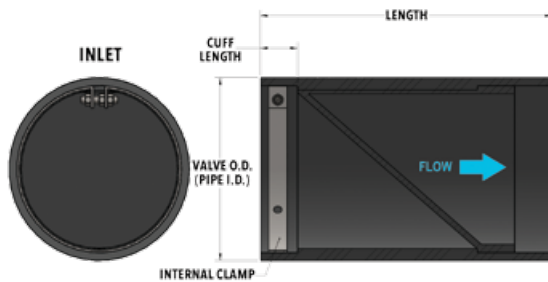
Upstream Clamp
