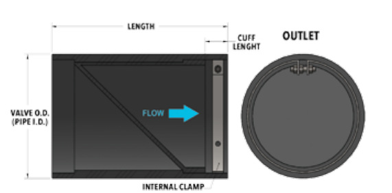
Downstream Clamp
