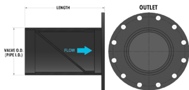
Downstream Flanged
