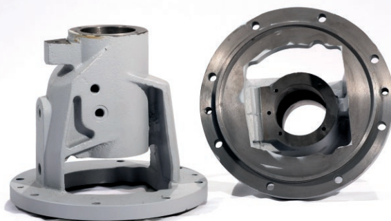
Bearing brackets and support for pumps
