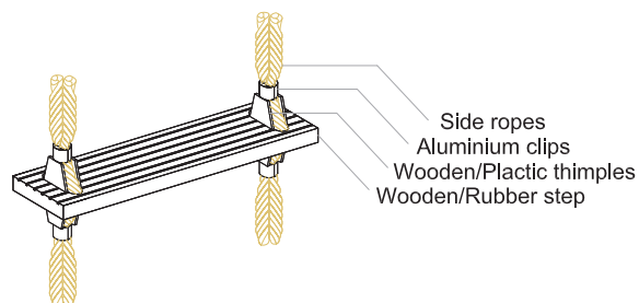
Detail A Typical step arrangement
