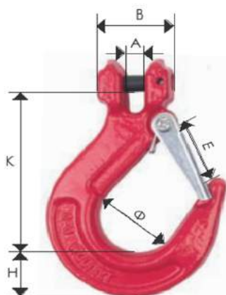
ZSW-012 G80羊角滑钩 (ZSW-012 G80 CLEVIS SLING HOOK WITH LATCH)
