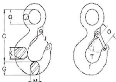
EYE HOOKS
