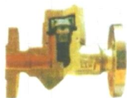
Thermostatic Steam Trap GG 25, GGG 40.3, C/S Flange, SW
