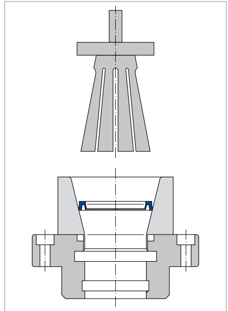
Fig. 23 Fitting of rod seals
