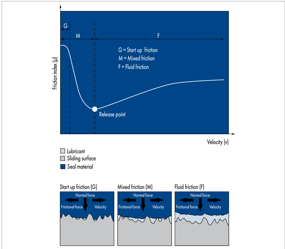
Fig. 12 Stribeck graph describes the dependency of the friction force on the speed
