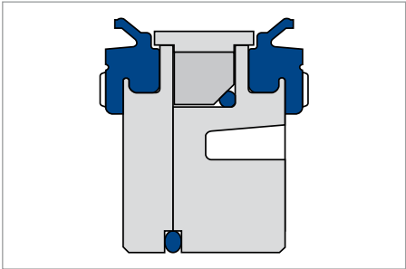
Merkel Complete Piston Pneuko M 310
