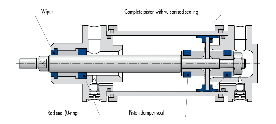
Fig. 3 Pneumatic cylinder II
