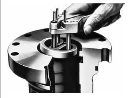
Fig. 21 Fitting tool for rod seals
