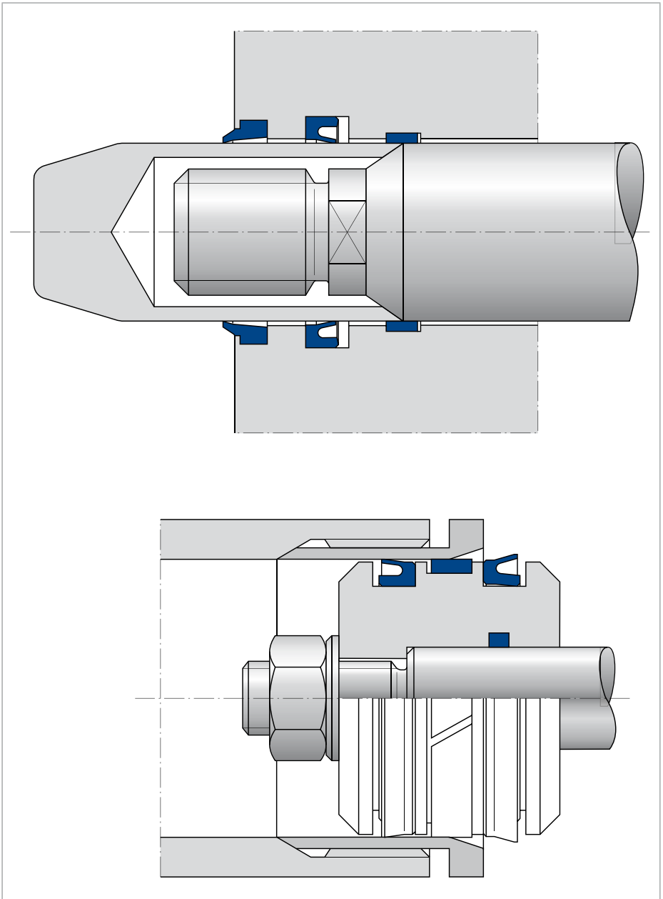
Fig. 19 Covering threads when mounting seals
