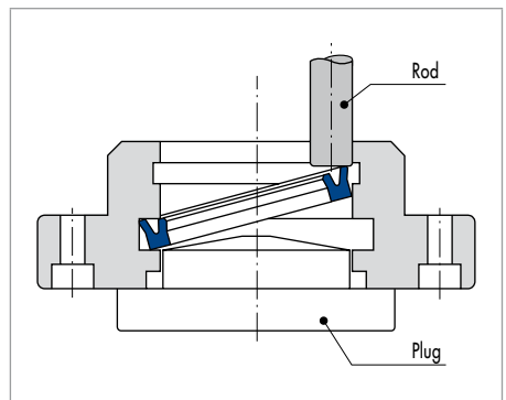
Fig. 24 Fitting aid for rod seals
