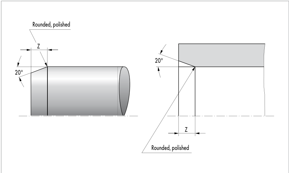
Fig. 18 Chamfering rods and pipes
