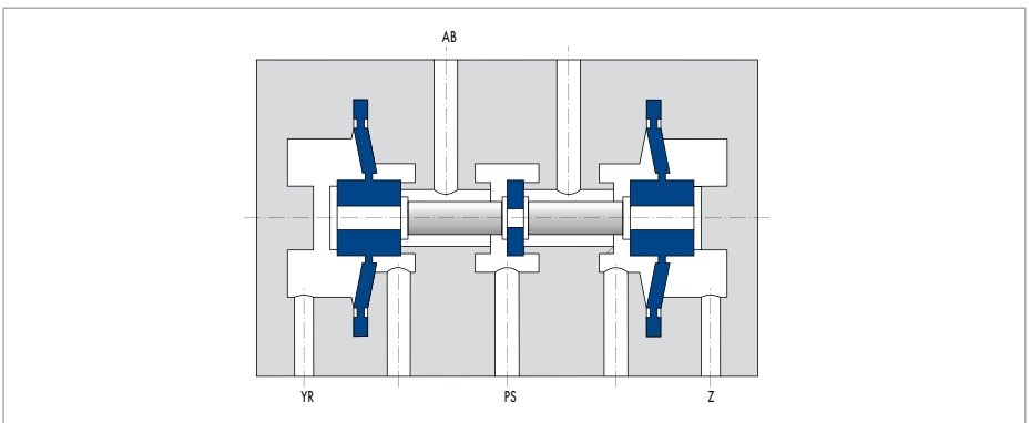
Fig. 8 Pneumatic 5/2-way valve
