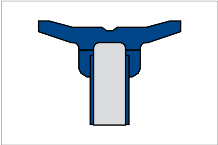
Merkel Complete Piston TDUOP with Venting Passages
