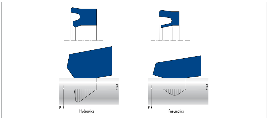
Fig. 10 Different lip geometry and pressure distribution with hydraulics and pneumatics
