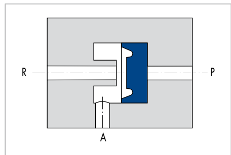
Fig. 6 Pneumatic quick-venting valve
