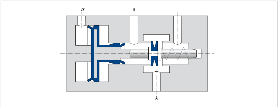
Fig. 7 Pneumatic 3/2-way valve
