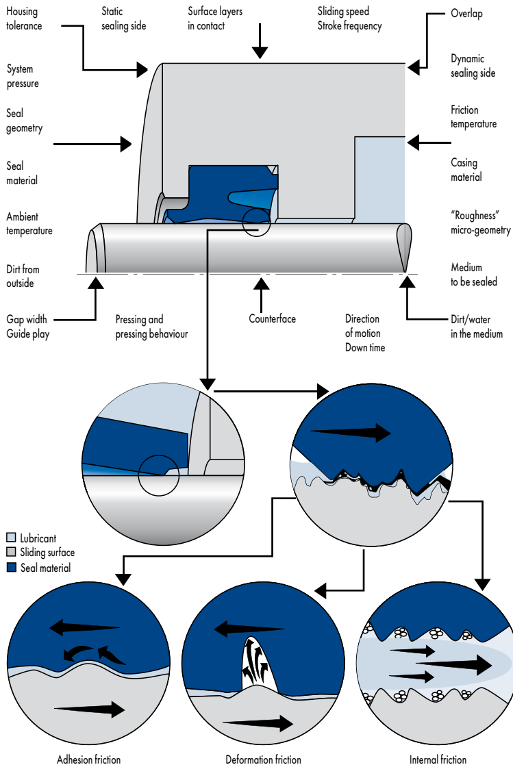
Fig. 11 Basic influences on the tribosystem
