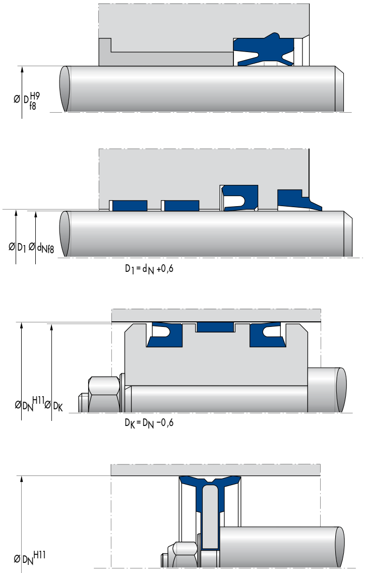
Fig. 16 Fitting and tolerances for seals and guides
