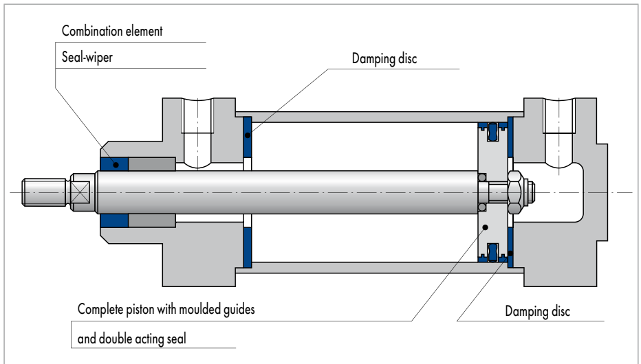
Fig. 1 Pneumatic cylinder I
