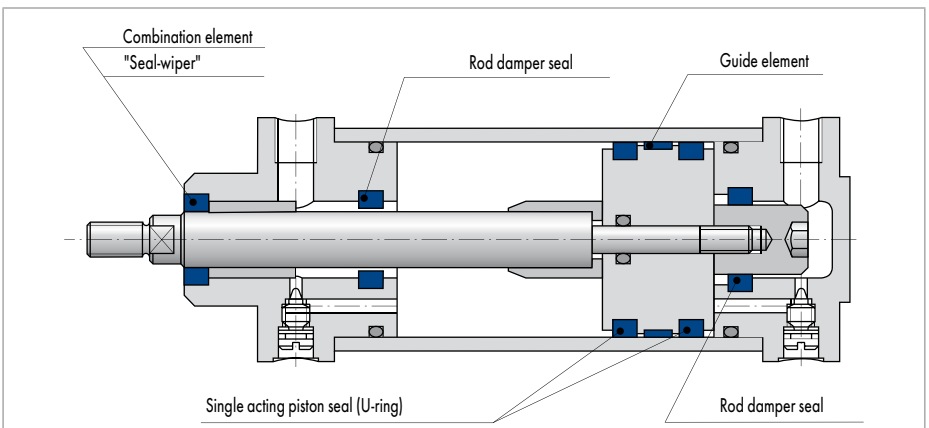
Fig. 4 Pneumatic cylinder III
