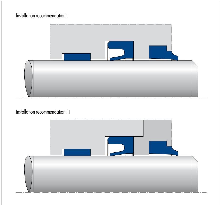
Fig. 20 Fitting types of rod seals
