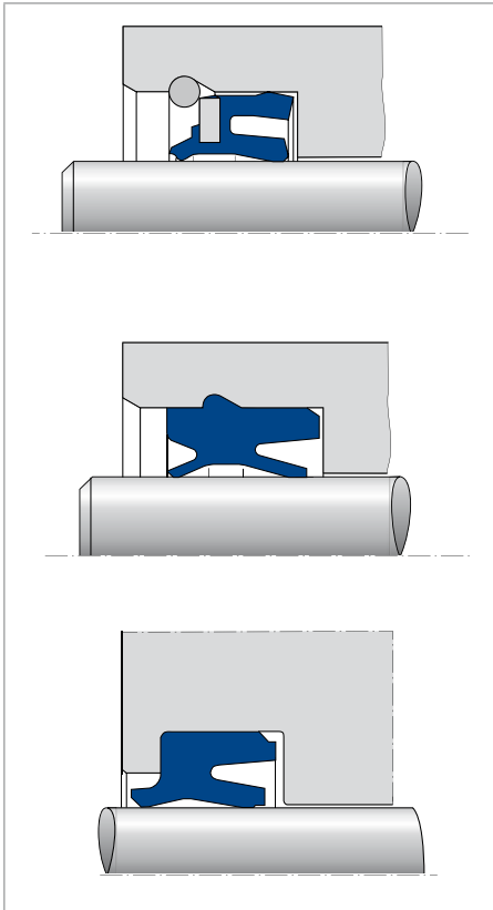
Fig. 25 Fitting of combination components
