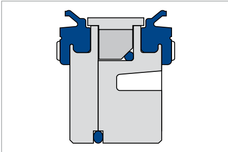
Merkel Complete Piston Pneuko M 210
