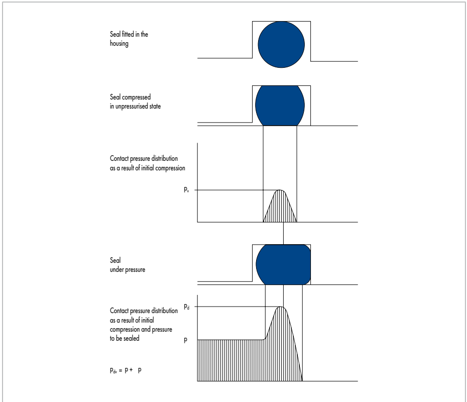
Fig. 9 Automatic sealing effect with elastic seals
