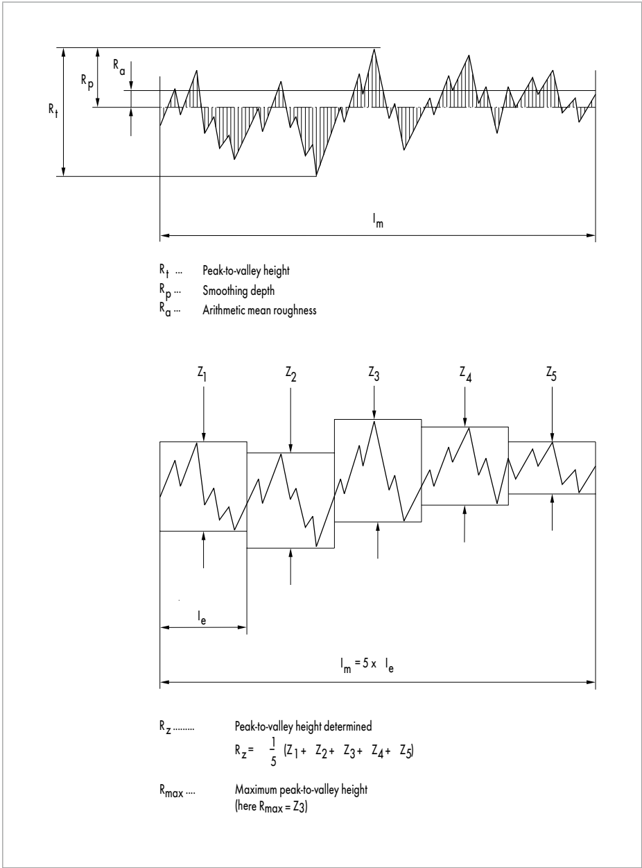
Fig. 17 Roughness terms
