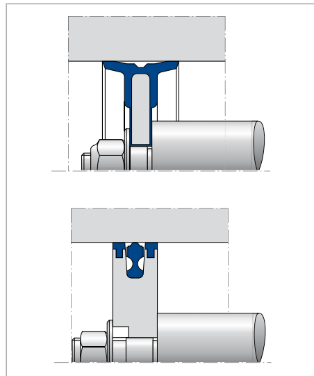
Fig. 28 Assembly of pneumatic complete pistons
