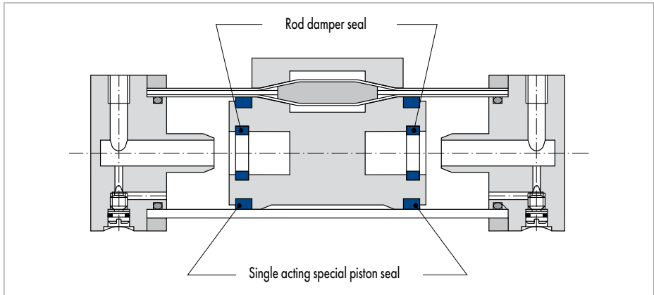
Fig. 5 Pneumatic cylinder without piston rod
