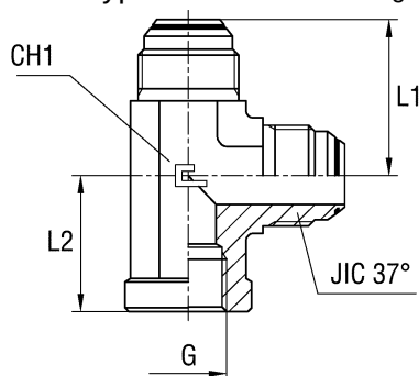
Type: 2030.. With O-ring
