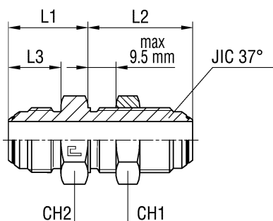
Type: 2020.. With O-ring
