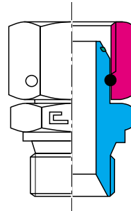
Product ready on stock. New 60° adapter with elastomeric seal designed by Cast.
