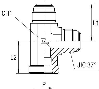
Type: 2031.. With O-ring
