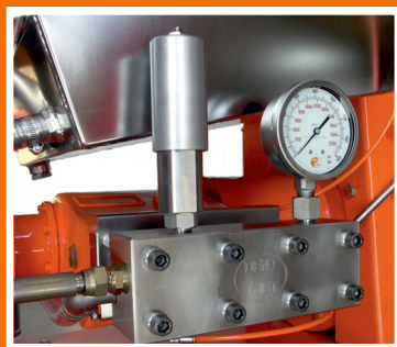
Stainless steel pump-head. Integrated cooling for plunger-seals.
