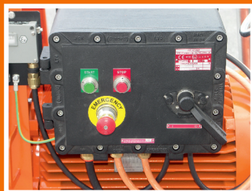
Cast electrical Eex box with main switch, star delta starter and overload relay.
