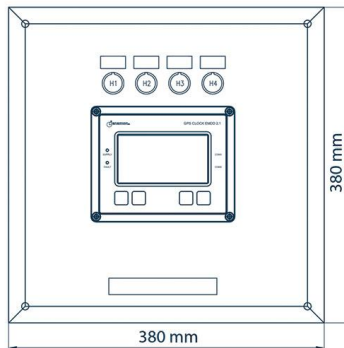
FRONT VIEW (Master Clock)
