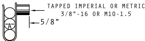
TRIPLE HANGER
