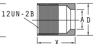
TUBE BODY
