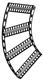
CABLE RACK HEAVY DUTY FLAT BEND 30°, 45°, 60°
