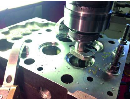
MEDIUM SPEED ENGINES – REBORING OF THE VALVE SEAT RINGS FOR THE OVERSIZE
