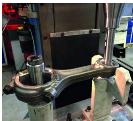
HIGH SPEED ENGINES - MACHINING OF THE CONNECTING ROD'S SMALL END BEARING
