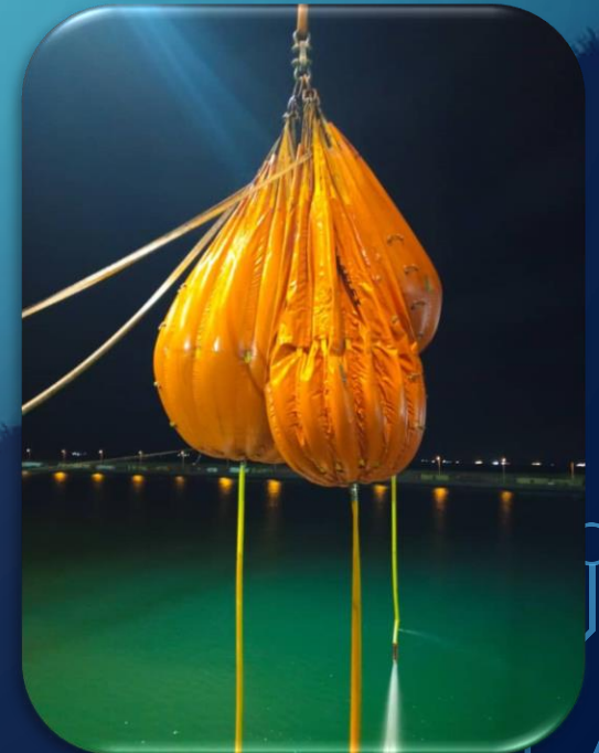
50 ton Load Test in Lome, Togo
