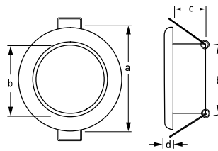
EuroLED 75 RGB/W
