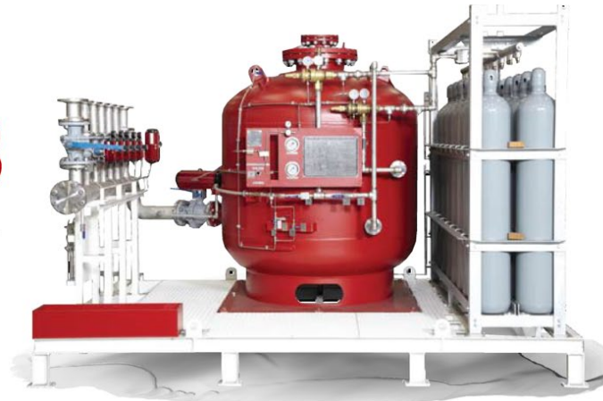
Mist SOL 6 Manual Valve 20A
