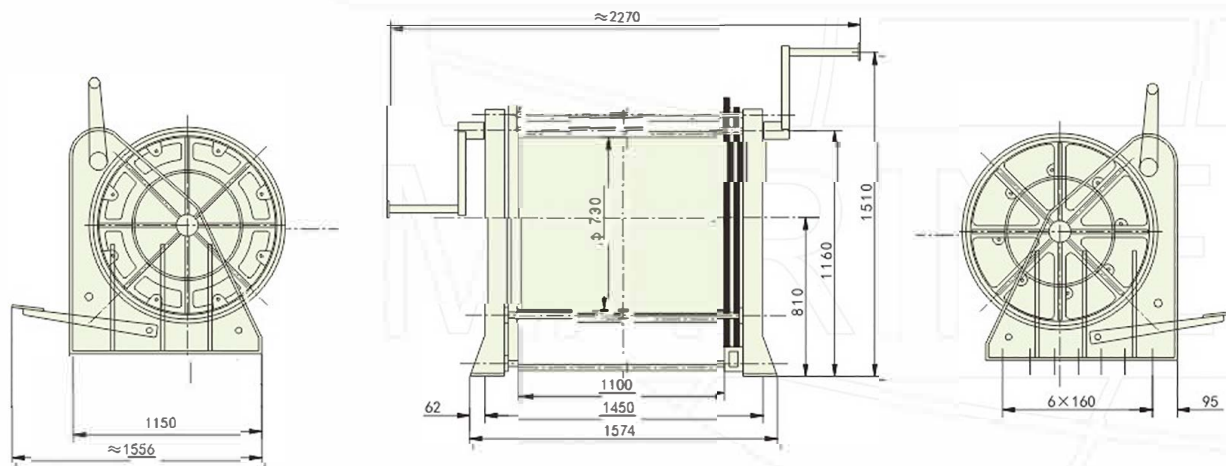
c型钢索卷车 Model C tightwire reel
