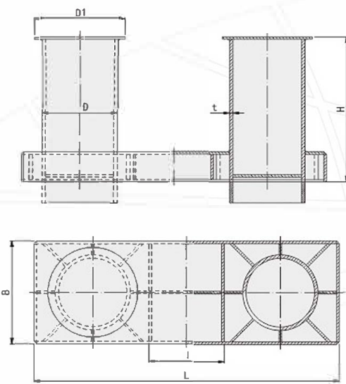
B型 - 嵌入带缆桩 Model B insert bollard bitt
