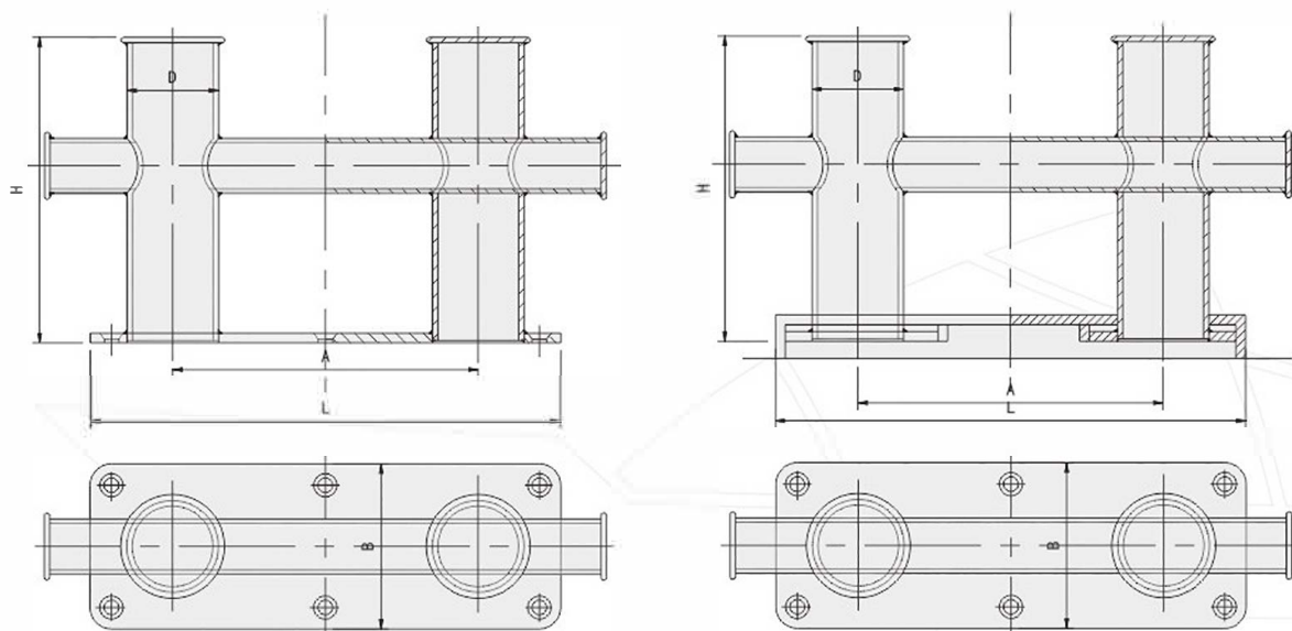
E型 - 双十字带缆桩 Model E double-cross bollard bitt
