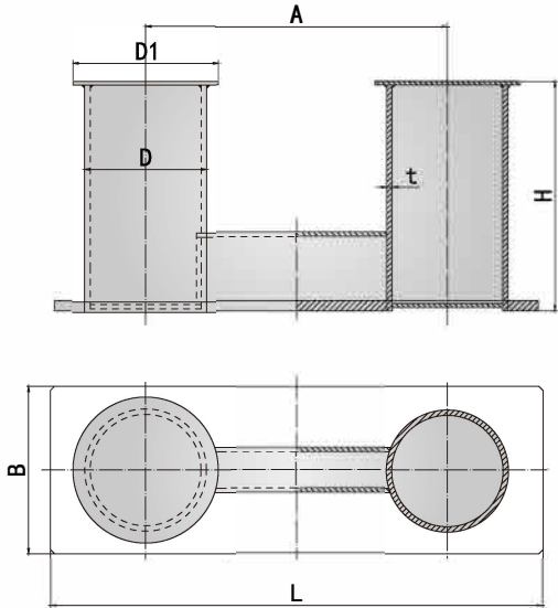
MODEL C BOLLARD BITT
