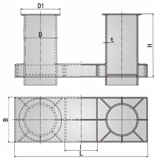
MODEL B INSERT BOLLARD BITT
