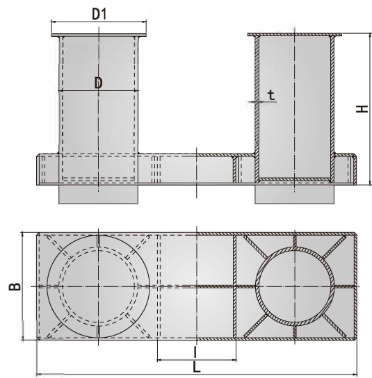
MODEL A COMMON BOLLARD BITT
