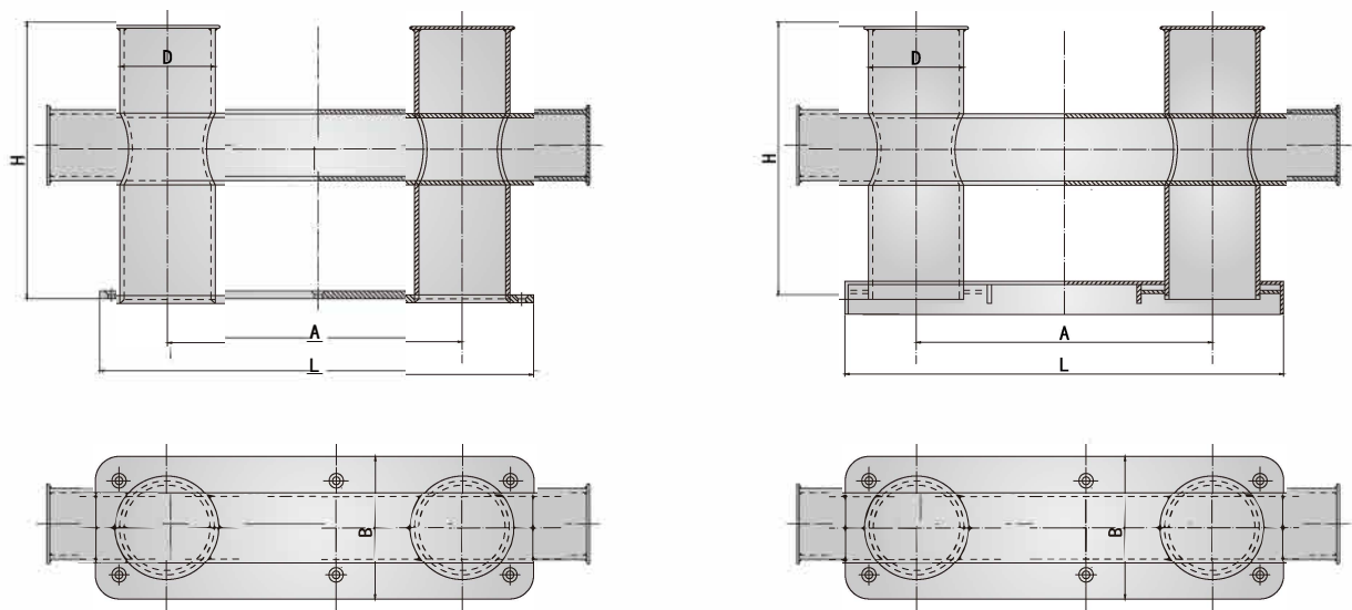
E型 - 双十字带缆桩 MODEL E DOUBLE-CROSS BOLLARD BITT
