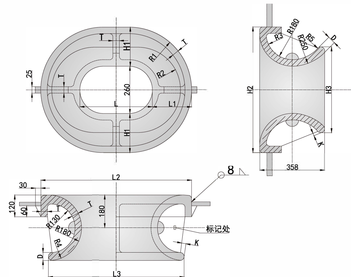
BC型导缆孔的型式和基本尺寸 TYPE BC CHOCK TYPE AND BASIC SIZE
