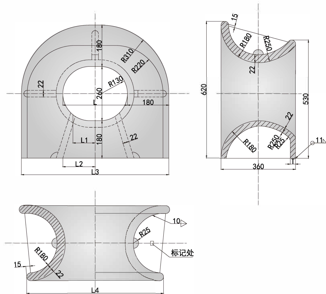
AP型导缆孔的型式和基本尺寸 TYPE AP CHOCK TYPE AND BASIC SIZE
