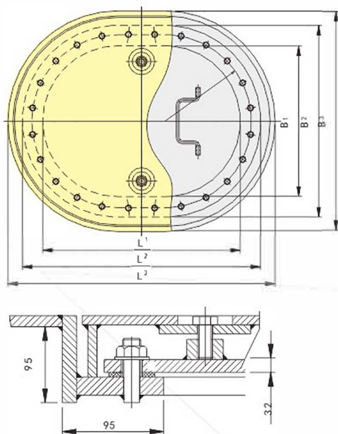
Model C - manhole cover
