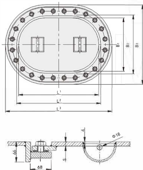
Model D - manhole cover
