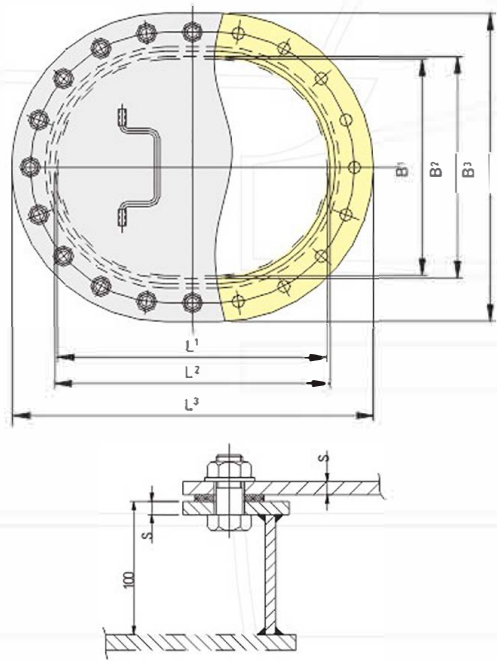
A 型-人孔盖 Model A - manhole cover
