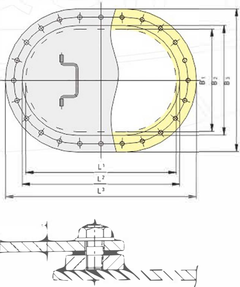
B 型-人孔盖 Model B - manhole cover
