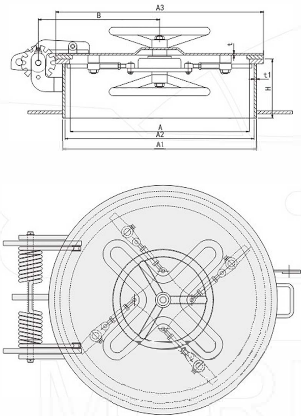
A型-耐压水密舱口盖 Model A - Pressure ant resist watertight hatch cover
