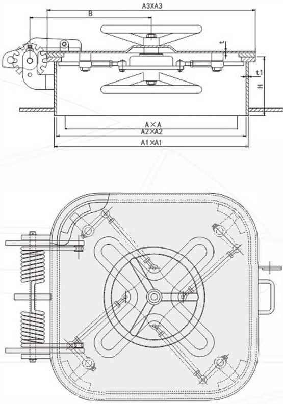
B型-耐压水密舱口盖 Model B - Pressure ant resist watertight hatch cover
