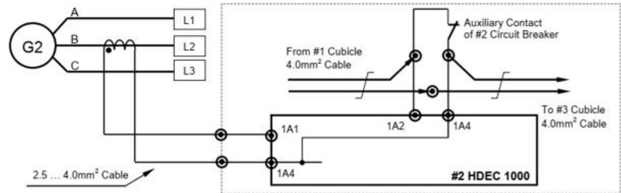
Figure 2-3 Typical Wiring Diagram for CCC (with single CT, Cubicle Mounting)
