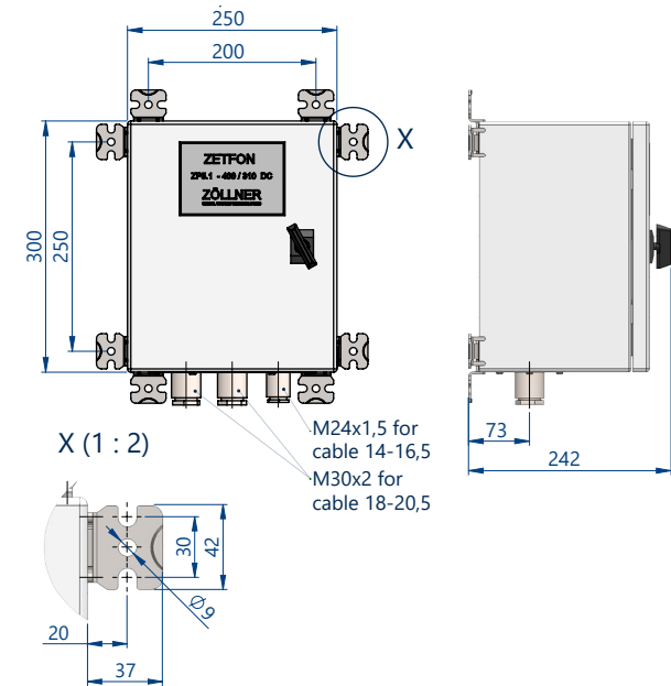
Control and amplifier unit ZP5.1 for ZET FON 400/310 DC
