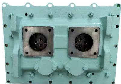
AIR COOLER
