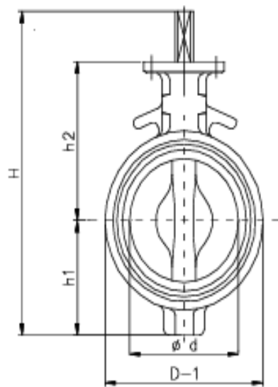
Wafer type.....Series 50
