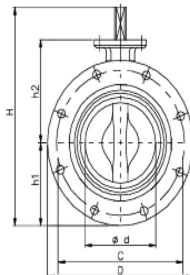
Flanged type...Series 55
