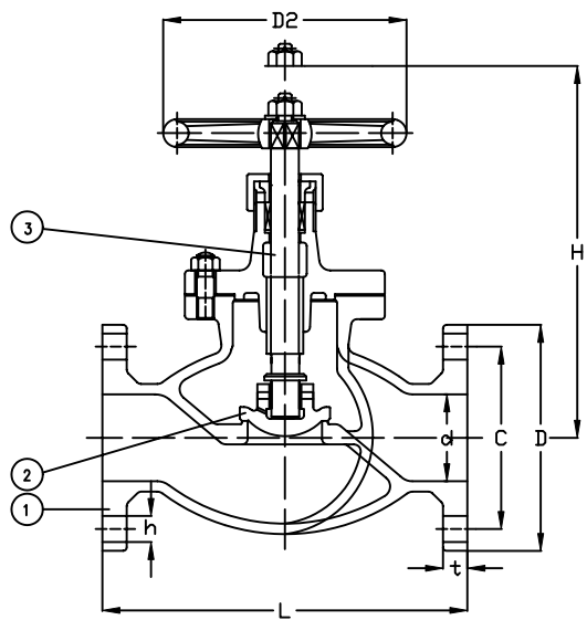
Bolted Bonnet for sizes 50A-65A
