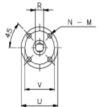
Top Flange to ISO5711
