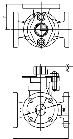
Three-Way Cock
